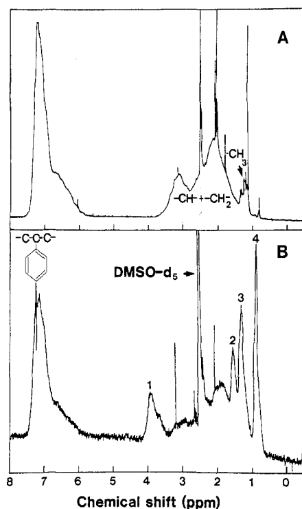
Figure 1. 1 H NMR (500 MHz) spectra of the fractionated (A) and its partially half-butyl-esterified SMA (B). Samples were dissolved at 5% in dimethyl- d 5 sulfoxide (Me 2 SO- d 5 ) at 40 °C. A few droplets of trifluoroacetic acid was added so that the peak due to H 2 O can be shifted outside the region shown in the figure. The peaks indicated by the numbers 1-4 in B are the signals of proton located in the corresponding positions of carbon in the butyl group. A broad bimodal peak appearing from 1.4 to 3.7 ppm in A is due to the methylene and tertiary carbon of the main chain. The peak due to the carboxyl group which appears at 12 ppm was not detected for SMA while it appeared for p-Bu-SMA (not shown).
