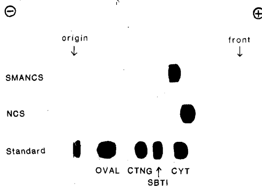
Figure 6. Disc gel electrophoresis in the presence of NaDodSO 4 at 0.2% in 0.025 M Tris-glycine buffer containing 2 mM EDTA, pH 8.3. Standard proteins and their molecular weight (in parentheses) are as follows: OVAL, ovalbumin (48 000); CTNG, chymotrypsinogen (24 000); SBTI, soybean trypsin inhibitor (20 000); CYT, cytochrome c (14 000); NCS, neocarzinostatin (12 000).
